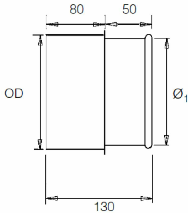
QF Machine adapter dimensions
