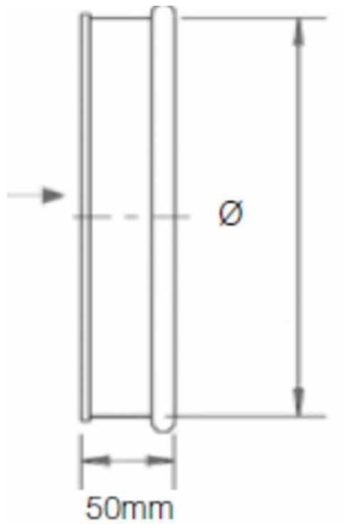
QF End Cap Dimensions, 22012-XXX
